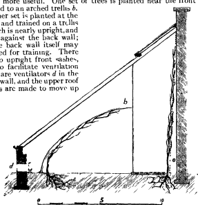
FIG. 8.—Peach House.
