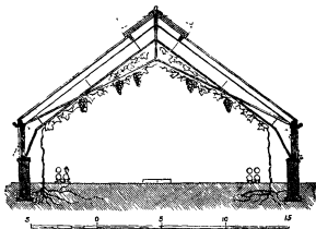
FIG. 7.—Span-Roofed Vinery.
