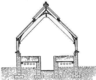
FIG. 9.—Forcing House.
