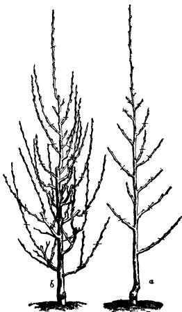
FIG. 28.—Pyramid Pruning.
