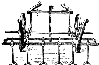
FIG. 3.—Martin's General Purpose Steerage Horse Hoe.
