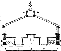
FIG. 4.—Section of Plant Stove.
